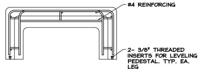
SMALL BENCH REINFORCING- ELEVATION
