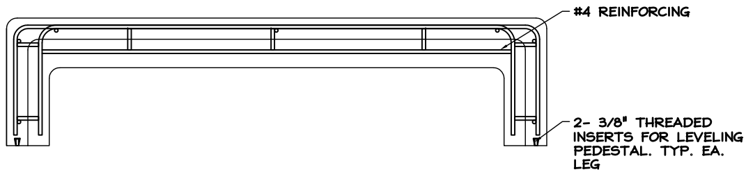
BENCH REINFORCING- ELEVATION
