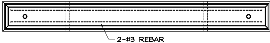
STANDARD 6'-PLAN DETAIL
