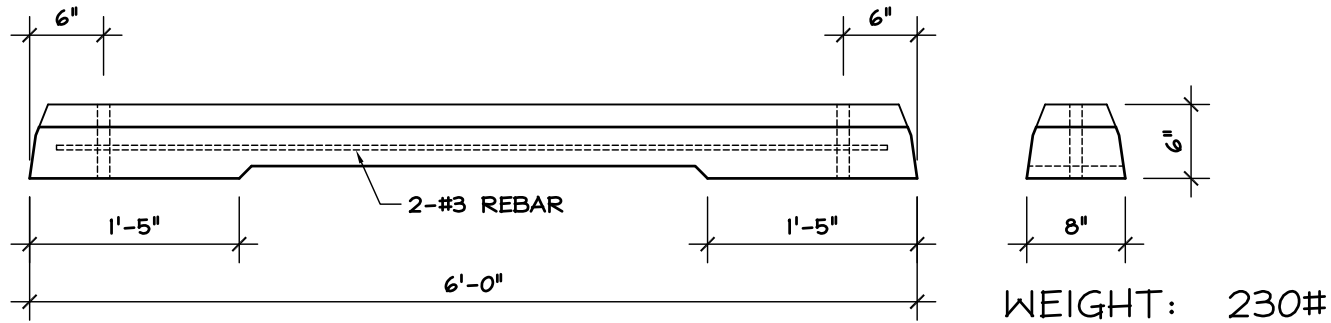
STANDARD 6'-ELEVATION DETAIL
